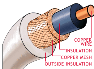
Cable coaxial
